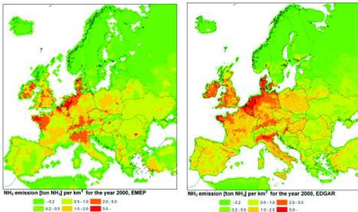
Fig. 4. Spatial distributions of annual NH 3 emissions in Europe for the year 2000 based on: (left) EMEP at 50 km × 50 km to the (right) EDGAR at 0.1° × 0.1°.
