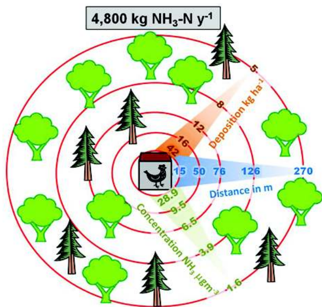
Fig. 9. Farm scale NH 3 emission and deposition, illustrating the rapid fall-off in deposition levels with distance from source (adapted from Fowler et al., 1998 and modified from version presented in Simpson et al., 2011).
