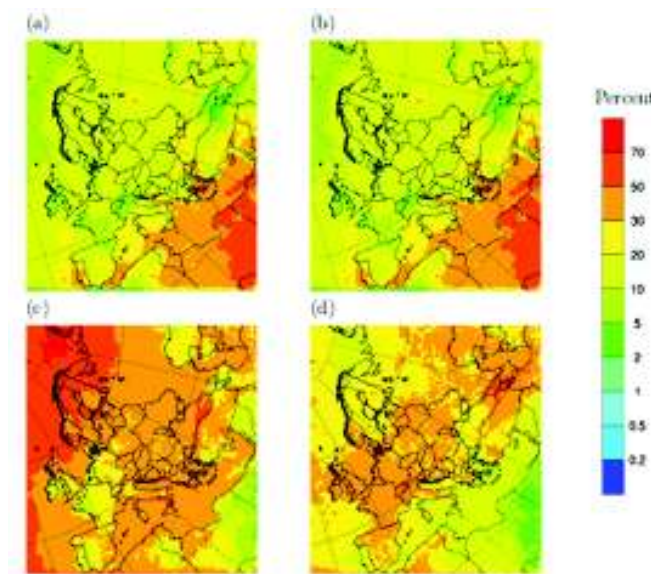
Fig. 11. Calculated percentage contributions to total nitrogen deposition for the year 2009: (a) dry deposition of oxidised N_r ; (b) dry deposition of reduced N_r ; (c) wet deposition of oxidised N_r ; (d) wet deposition of reduced N_r . Calculations with EMEP MSC-W model (Simpson et al., 2012).
